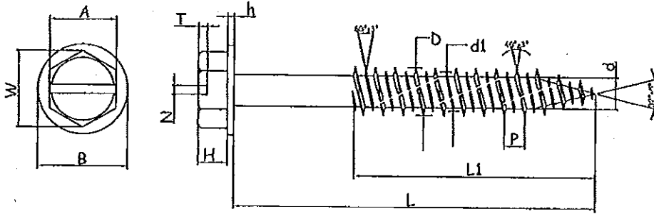
SLOTTED HEX WASHER HEAD CONCRETE ANCHOR
