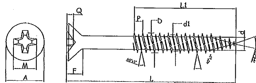
PHILIPS FLAT HEAD CONCRETE ANCHOR
